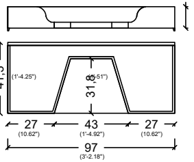
TOP VIEW DRAWER
