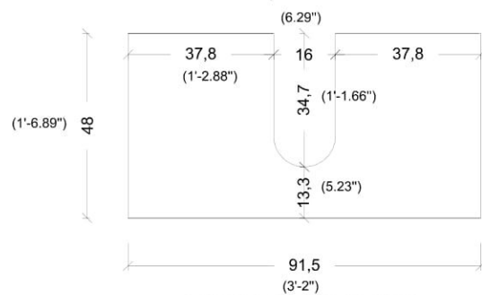
CABINET BACKING
